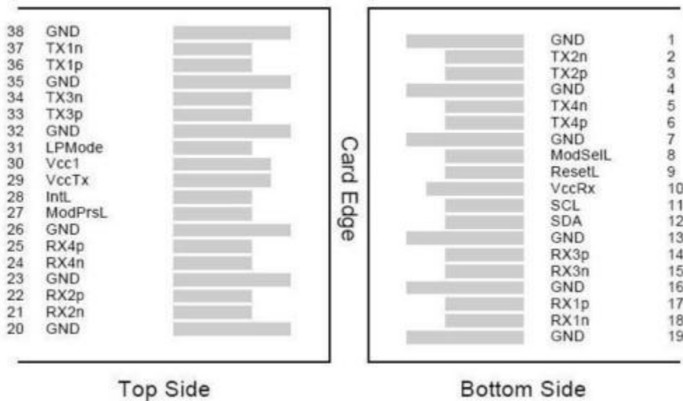
Figure 7.1 QSFP28 Transceiver Electrical Pad Pinout
