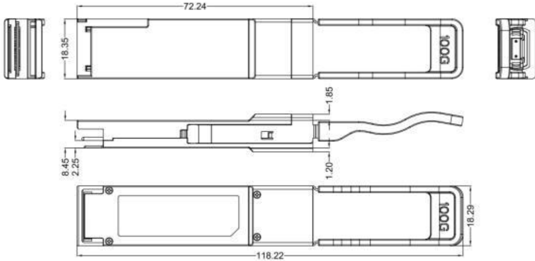
Figure 8.1 Package dimensions
