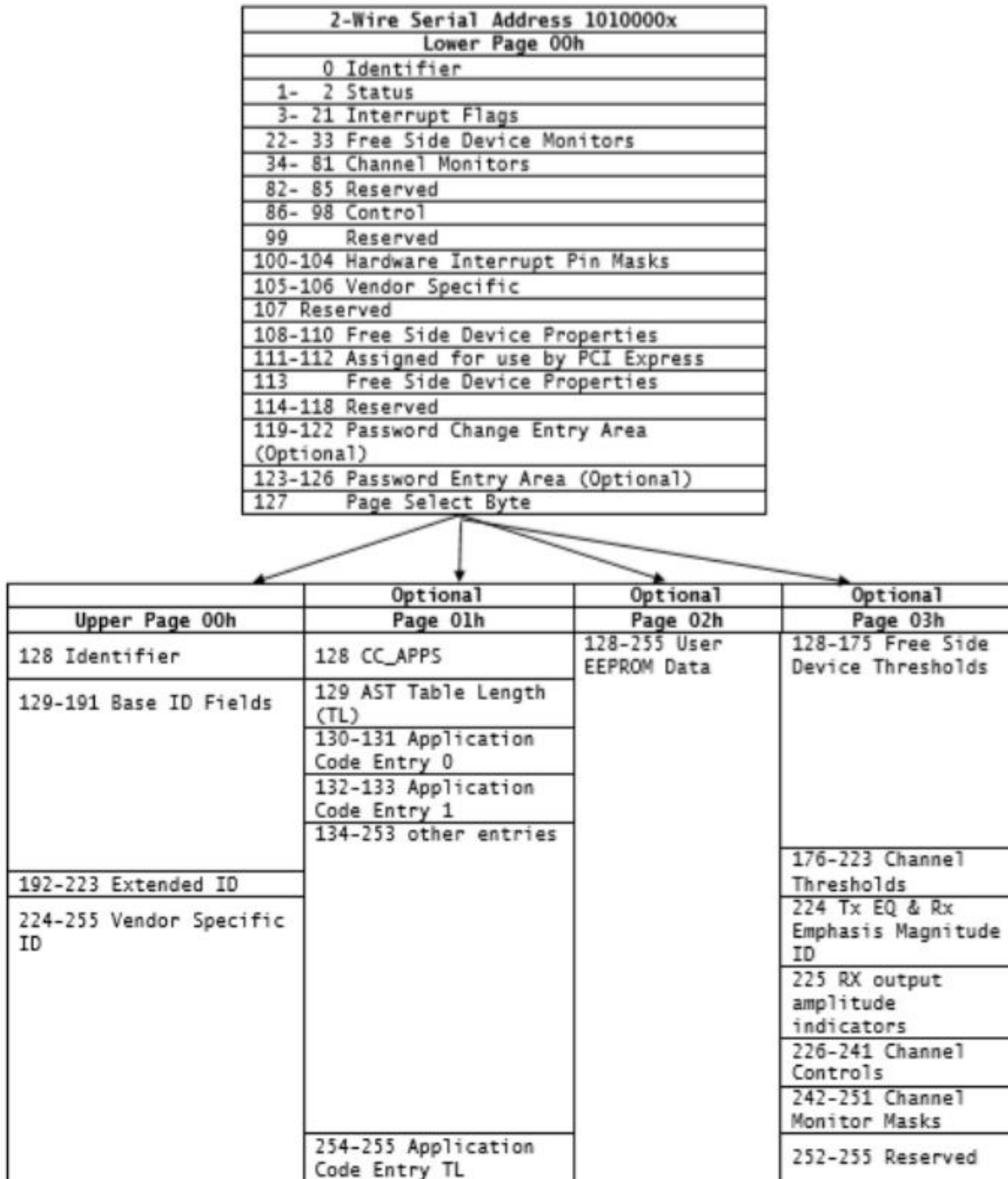
Figure 6.1 QSFP28 Memory Map
