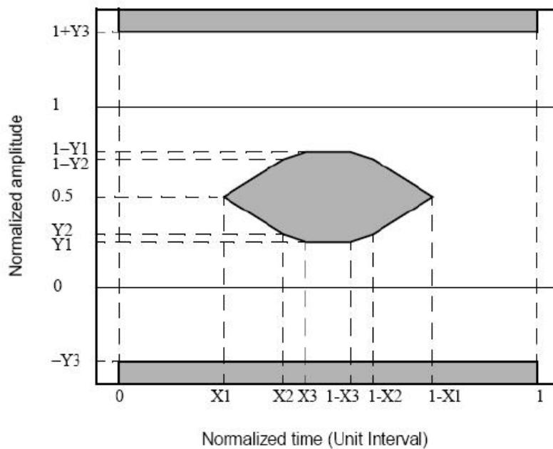
Figure1. EyeMaskDefinition
